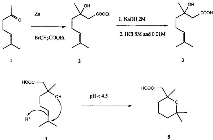
Scheme I: synthetic pathway to racemic hydroxy-3-citronellic acid
