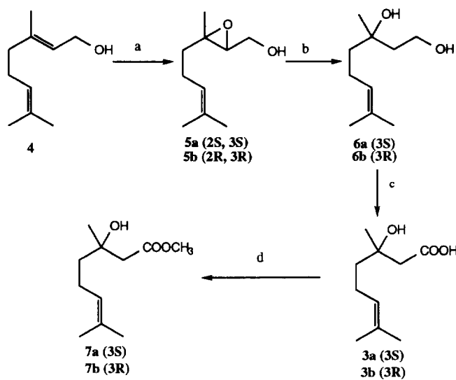
Scheme II: enantioselective pathway to (3R and 3S) methyl 3-hydroxy citronellate ( 7a and 7b )
